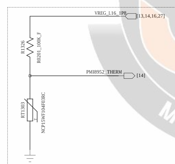
RT1303 is used for PMI surface temperature detect
