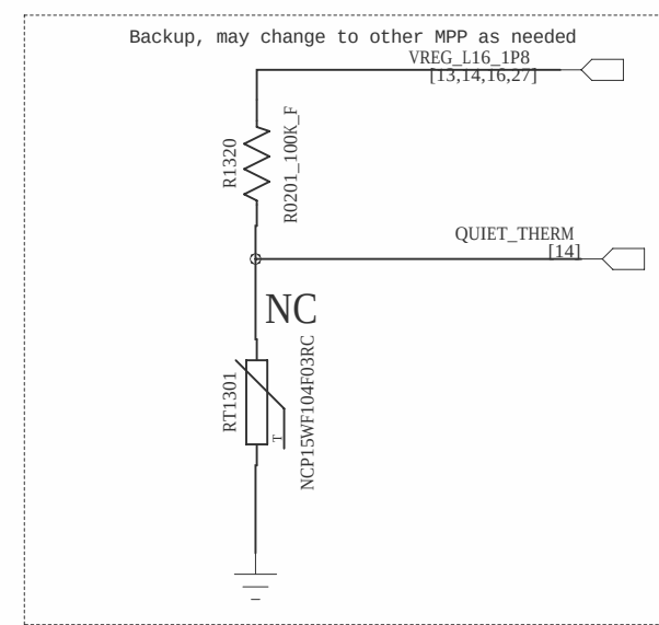
RT1301 is for CPU surface temperature detect
